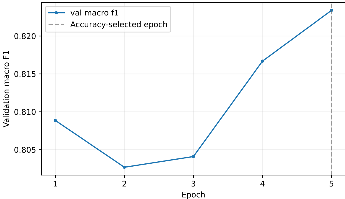
s37_convnext_control_strict_dev_seed42 | warm-start intervention
