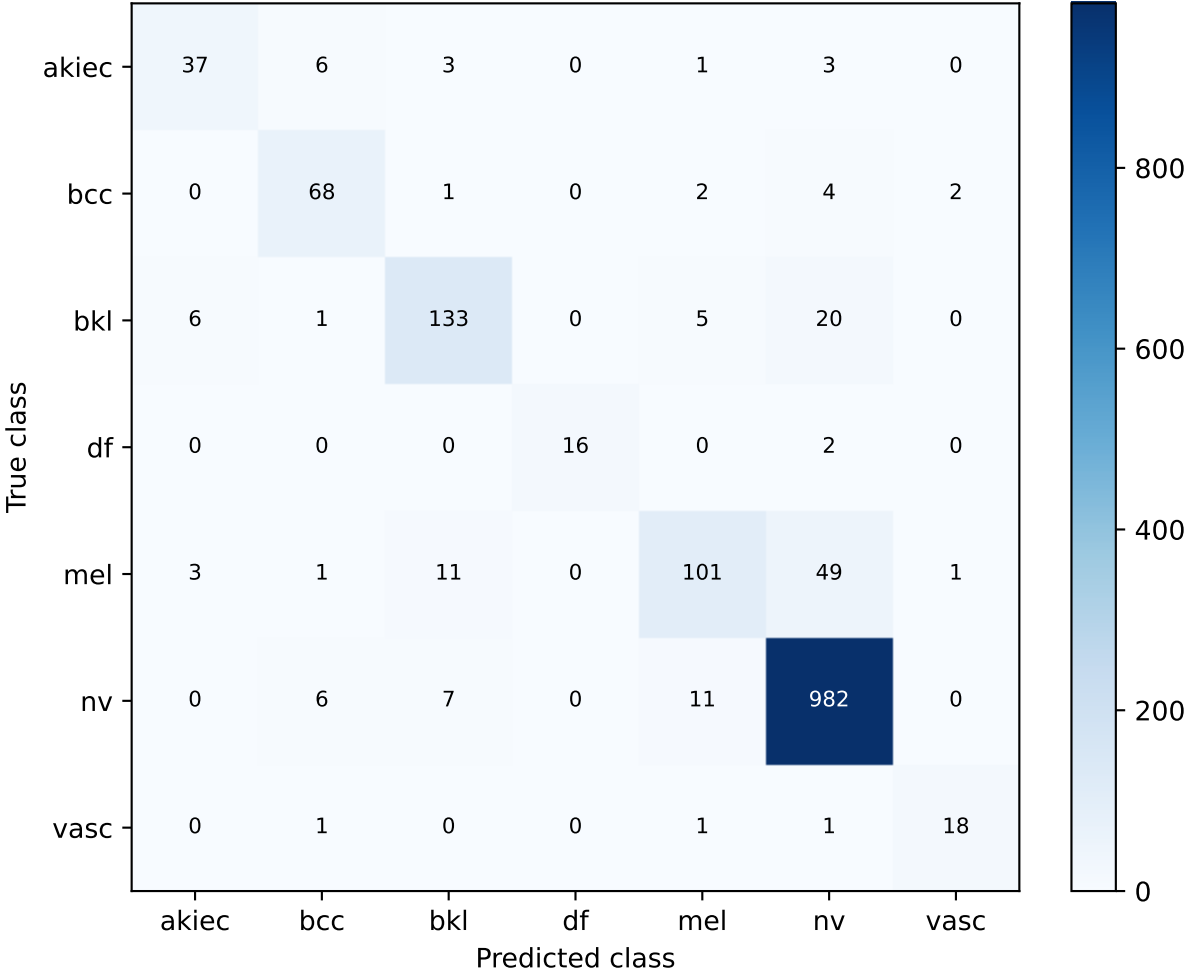
s38_convnext_melbkl_sampling_strict_dev_seed42 | fixed B0 + candidate + V2S Confusion matrix
