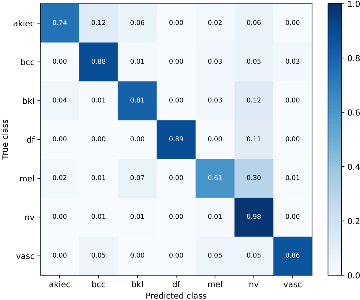
s38_convnext_melbkl_sampling_strict_dev_seed42 | fixed B0 + candidate + V2S Row-normalized confusion matrix
