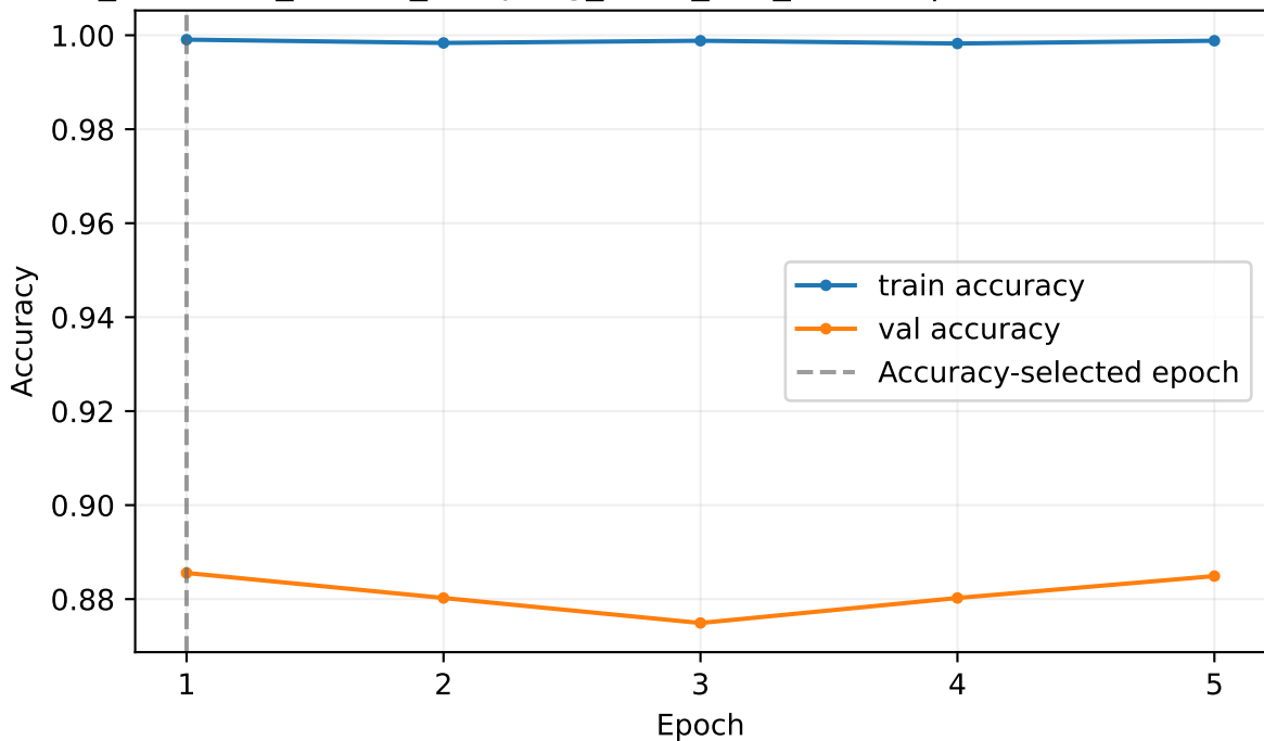
s38_convnext_melbkl_sampling_strict_dev_seed42 | warm-start intervention
