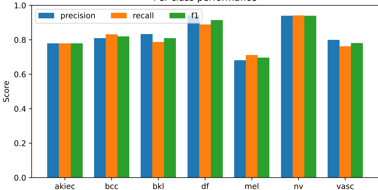
s38_convnext_melbkl_sampling_strict_dev_seed42 | post-test strict development Per-class performance
