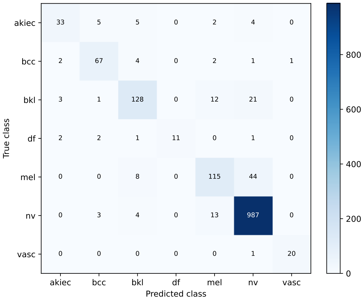
S91 DeiT III Base | exploratory validation Confusion matrix
