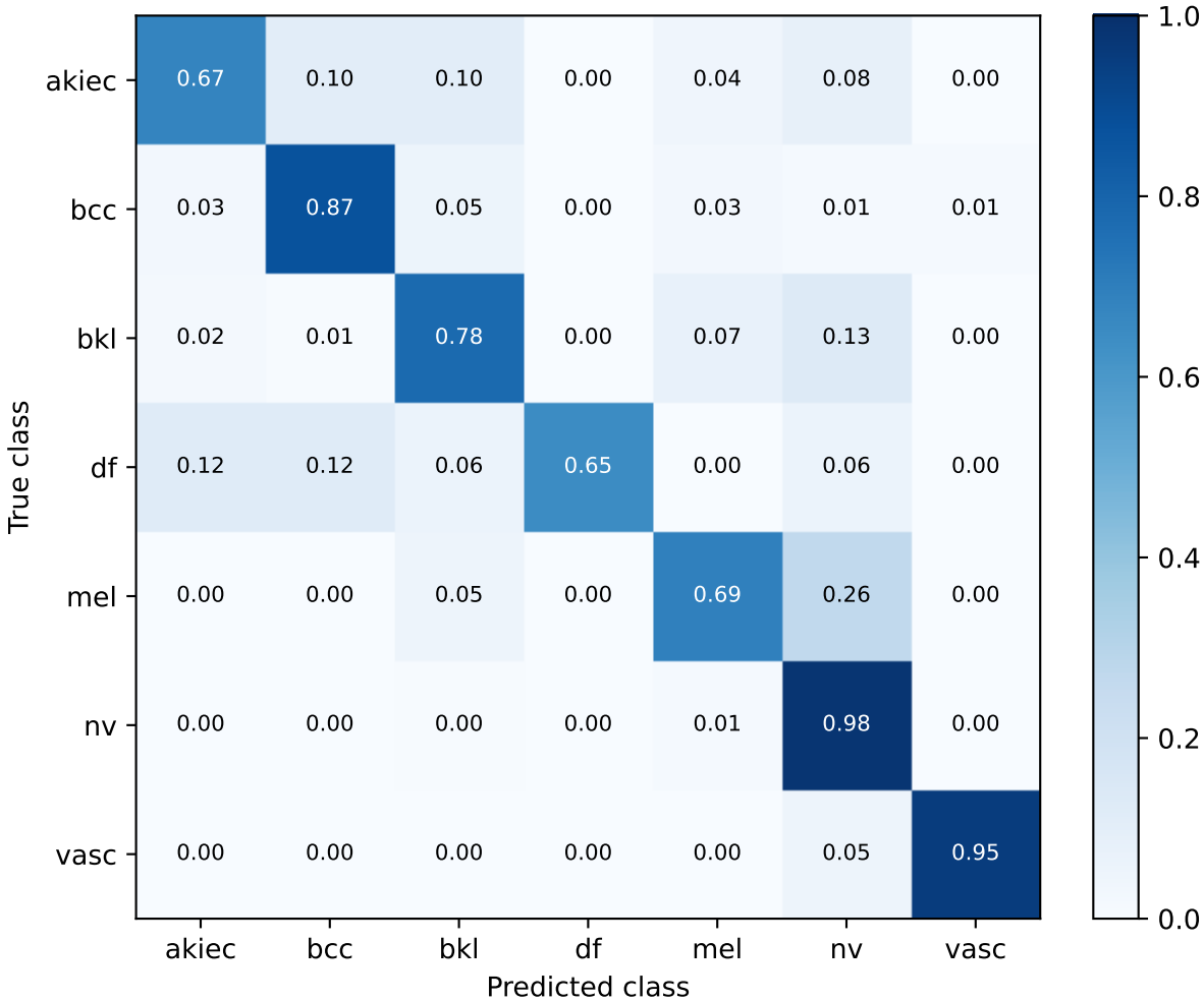
S91 DeiT III Base | exploratory validation Row-normalized confusion matrix
