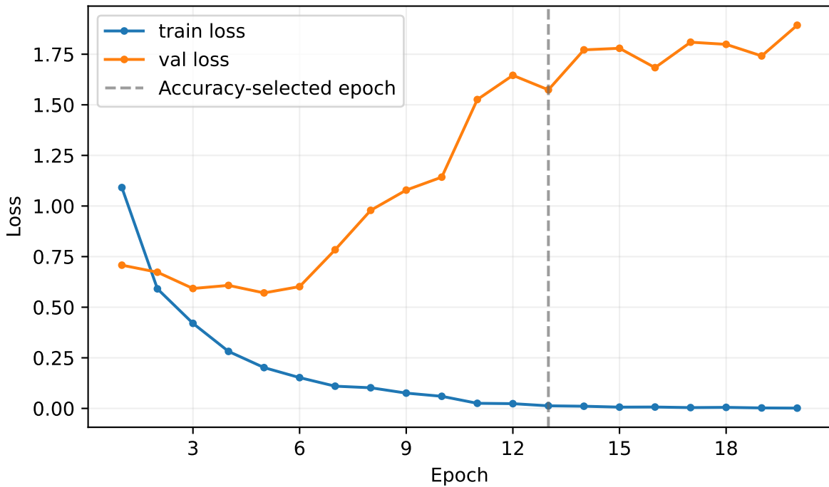
S91 DeiT III Base training
