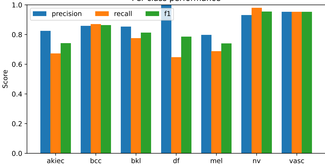
S91 DeiT III Base | exploratory validation Per-class performance
