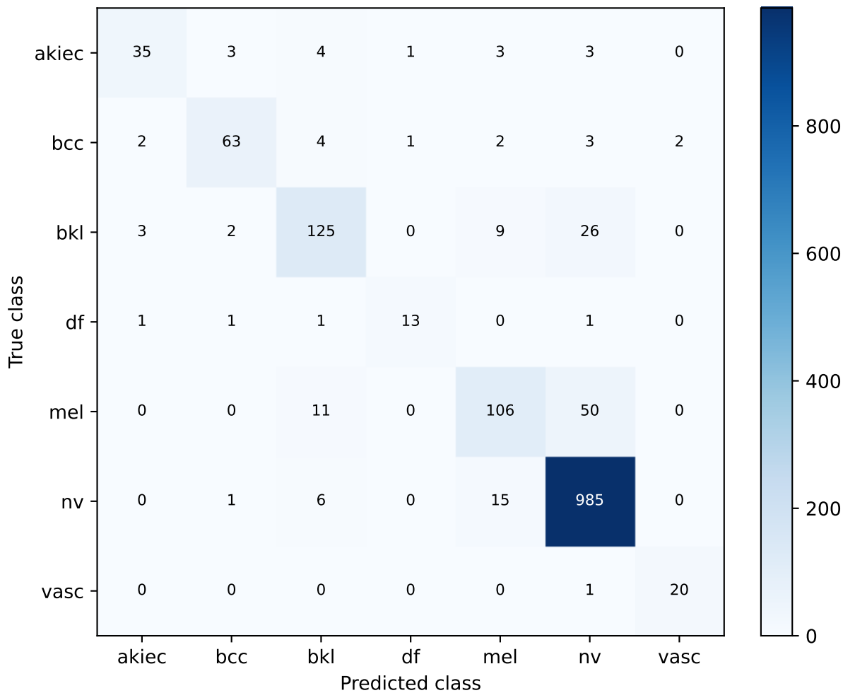
S91 DeiT III Base final committed epoch | exploratory validation Confusion matrix
