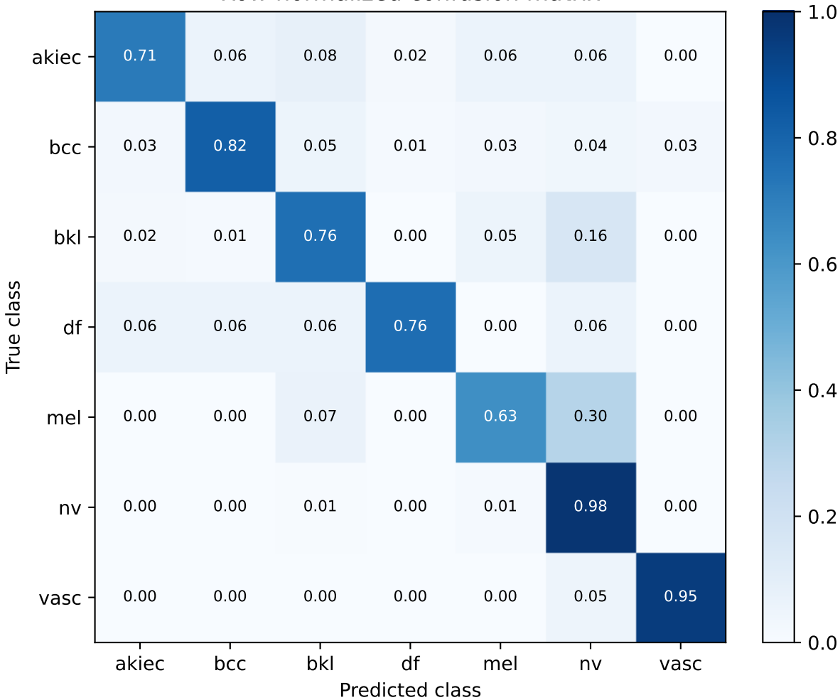
S91 DeiT III Base final committed epoch | exploratory validation Row-normalized confusion matrix
