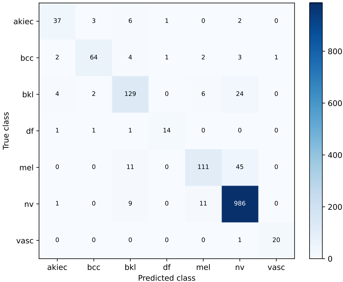
S91 DeiT III Base | exploratory_validation_macro_f1 Confusion matrix
