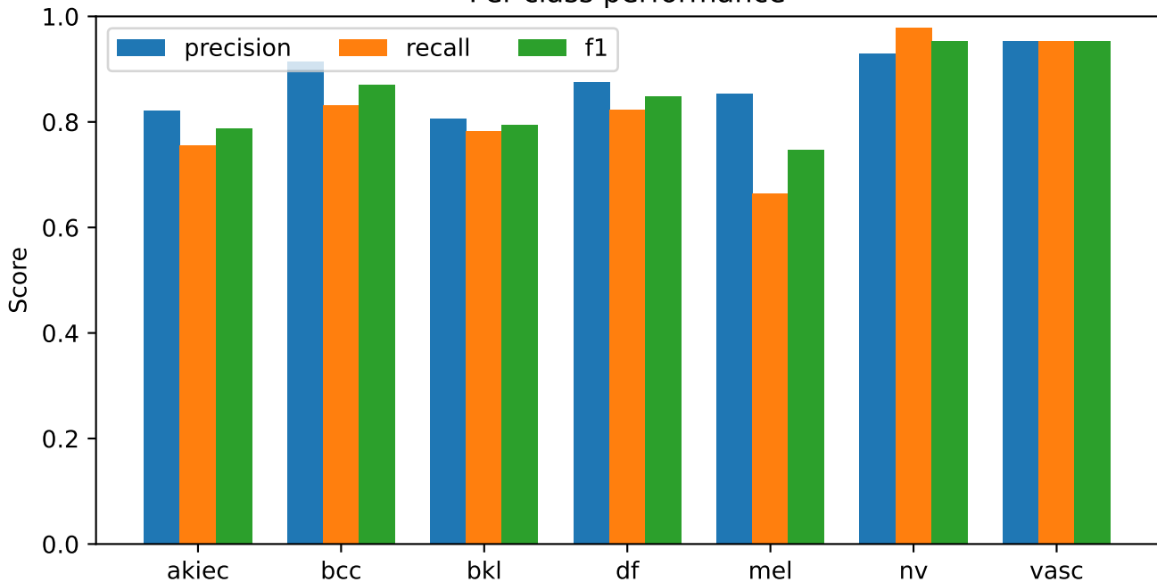
S91 DeiT III Base | exploratory_validation_macro_f1 Per-class performance
