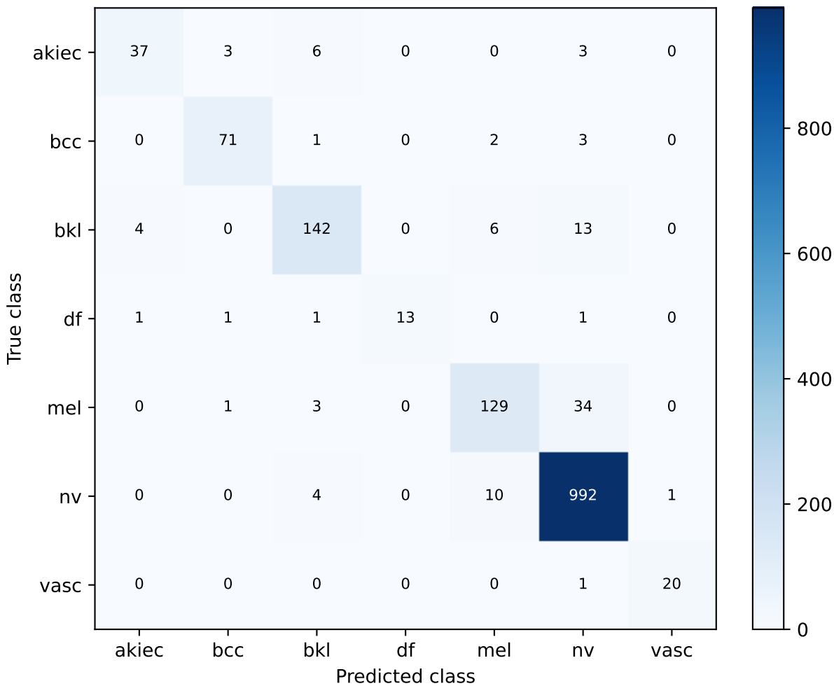
S94 S83 + both | exploratory validation Confusion matrix
