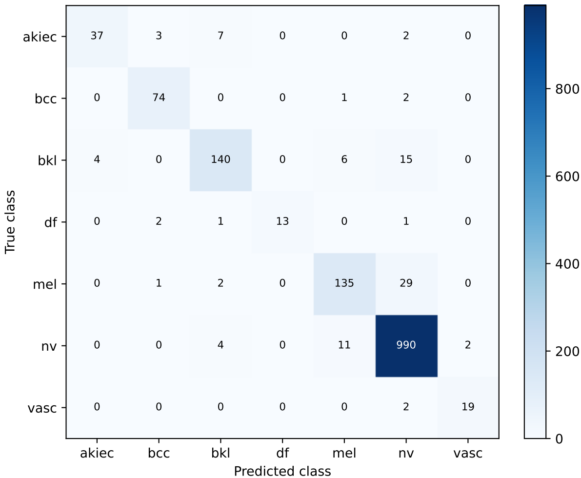
S92 S83 + swin | exploratory validation Confusion matrix
