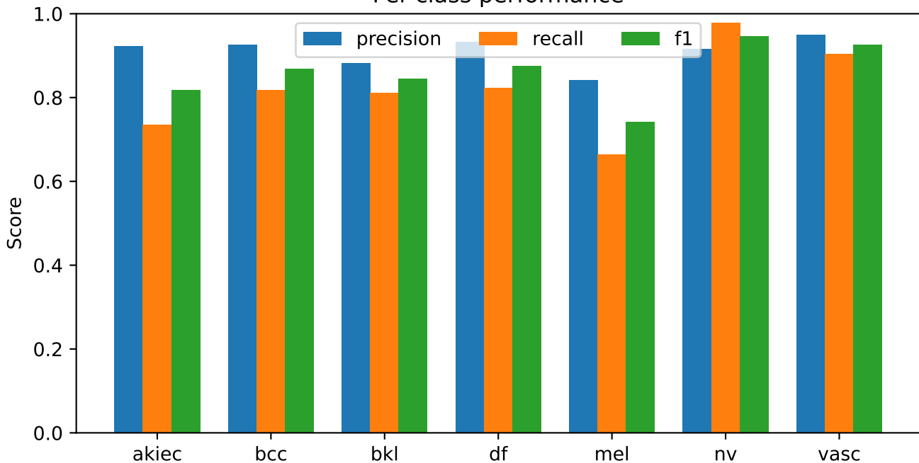
S89 Swin-Tiny | exploratory_validation_macro_f1 Per-class performance
