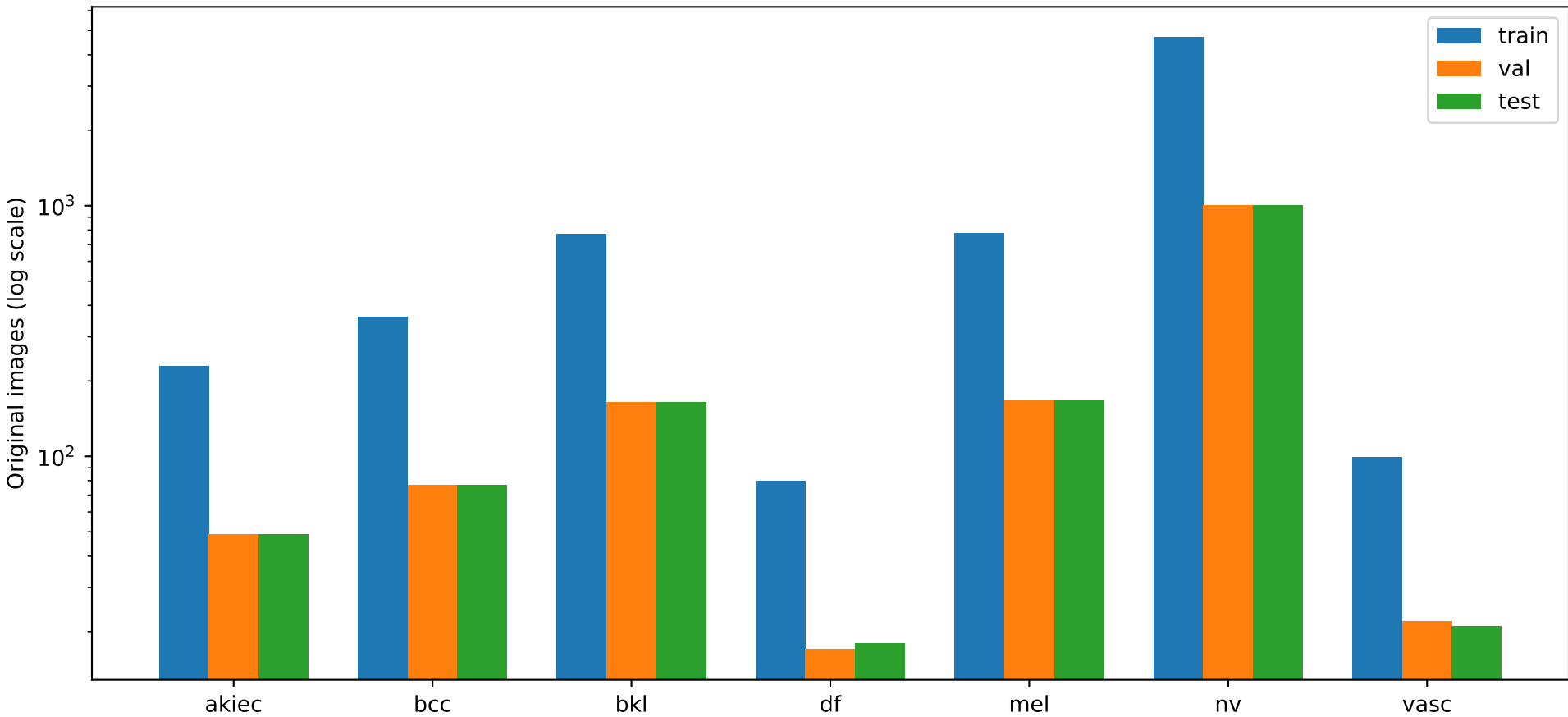
New image-level 70/15/15 study: natural class counts
