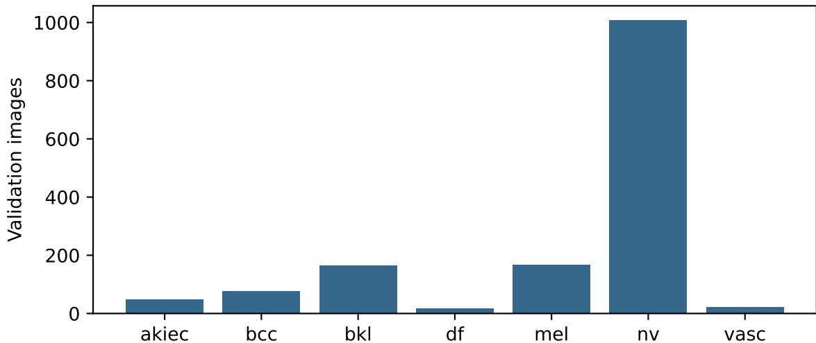
mobilenet_v3_large | exploratory_image_level validation Class support
