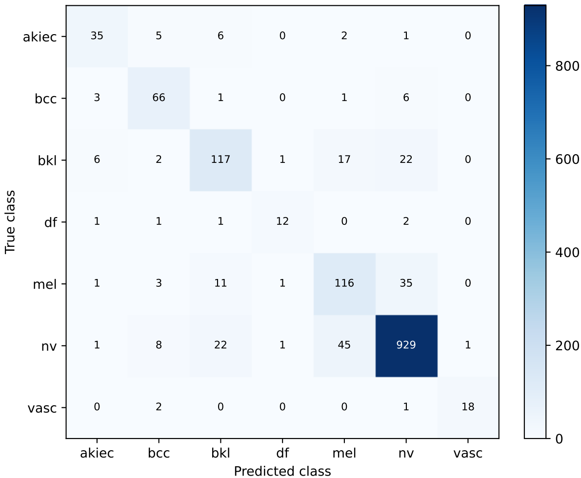
mobilenet_v3_large | exploratory_image_level validation Confusion matrix
