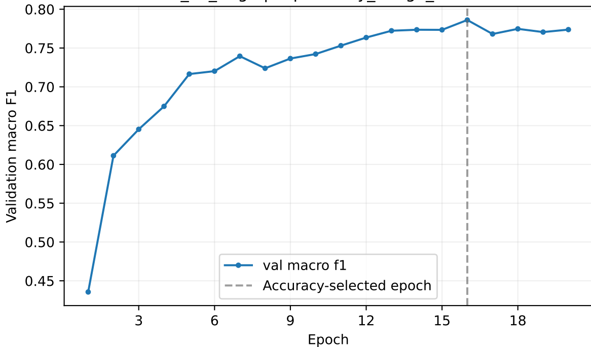
mobilenet_v3_large | exploratory_image_level validation
