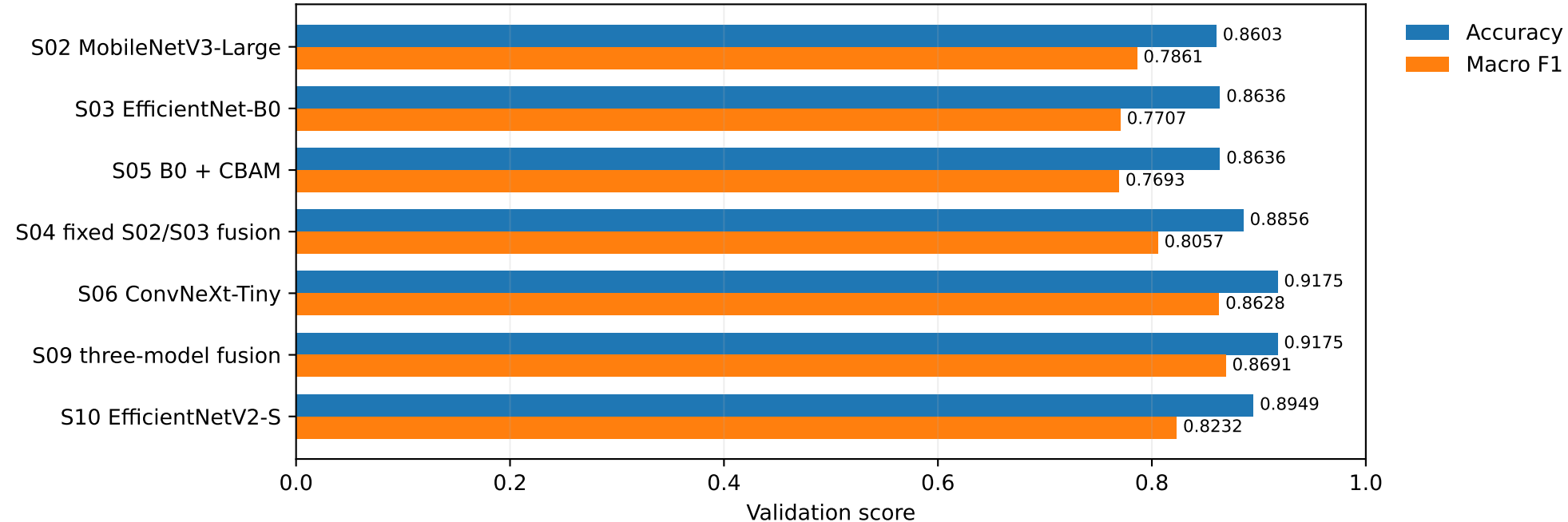
Same exploratory validation | accuracy winners and fixed fusions S10: unchanged AMP training; FP32 fallback at epochs 14/18/20; winner 15 AMP
