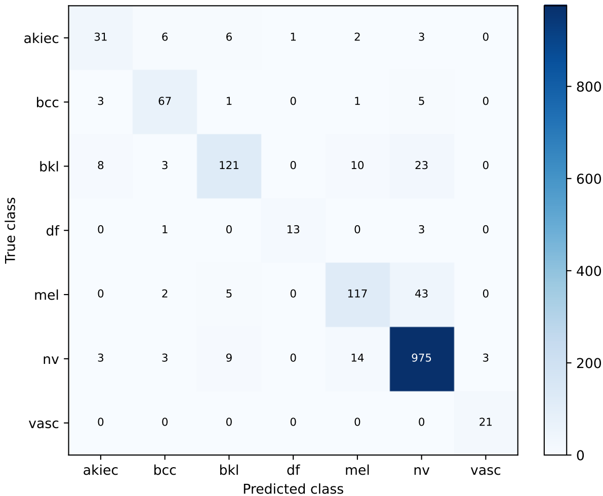
efficientnet_v2_s | exploratory_image_level validation Confusion matrix
