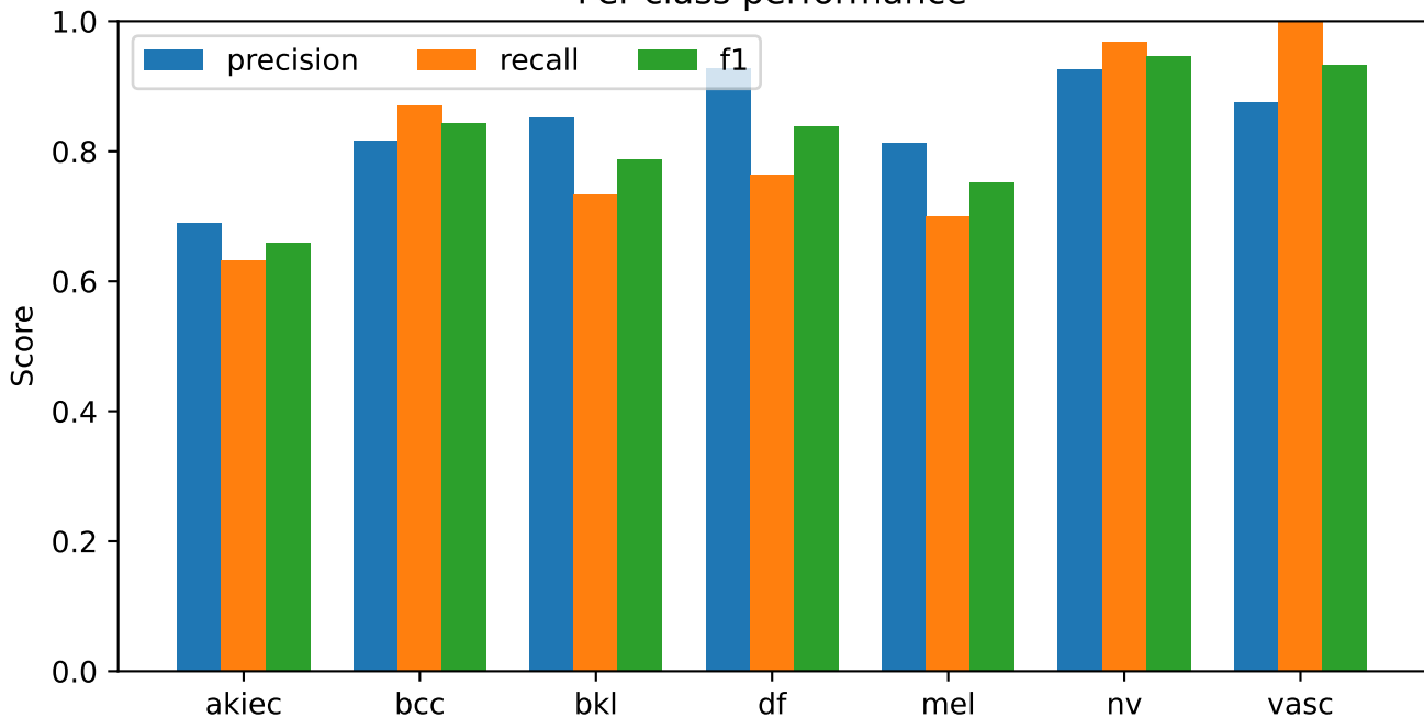
S10 EfficientNetV2-S | exploratory validation | macro-F1 winner Per-class performance
