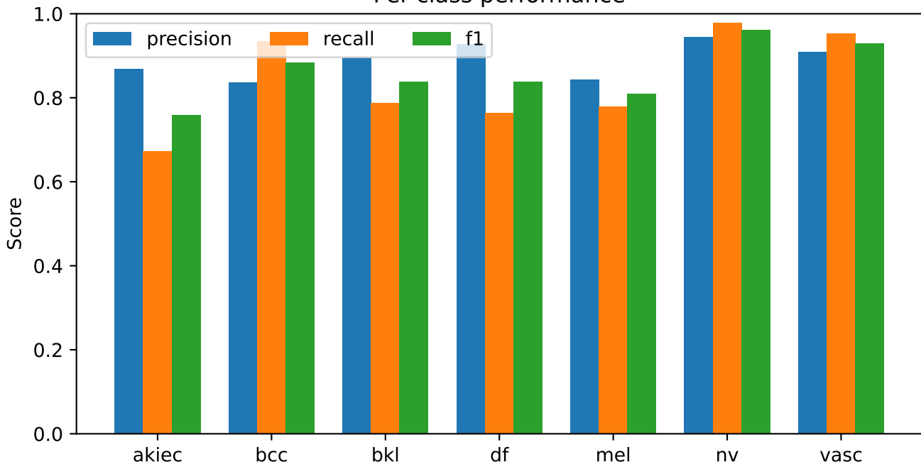
S11 fixed equal fusion | exploratory validation | no weight tuning Per-class performance
