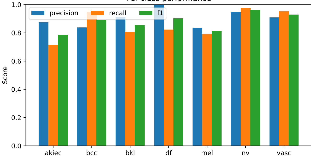
S12 fixed equal fusion | exploratory validation | no weight tuning Per-class performance
