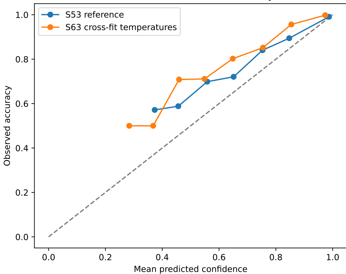
Fixed ten-bin ensemble reliability
