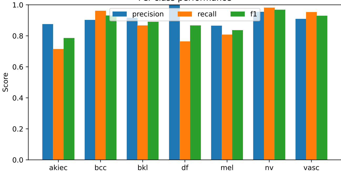
S63 equal calibrated fusion | held-out meta folds; exploratory CNNs Per-class performance
