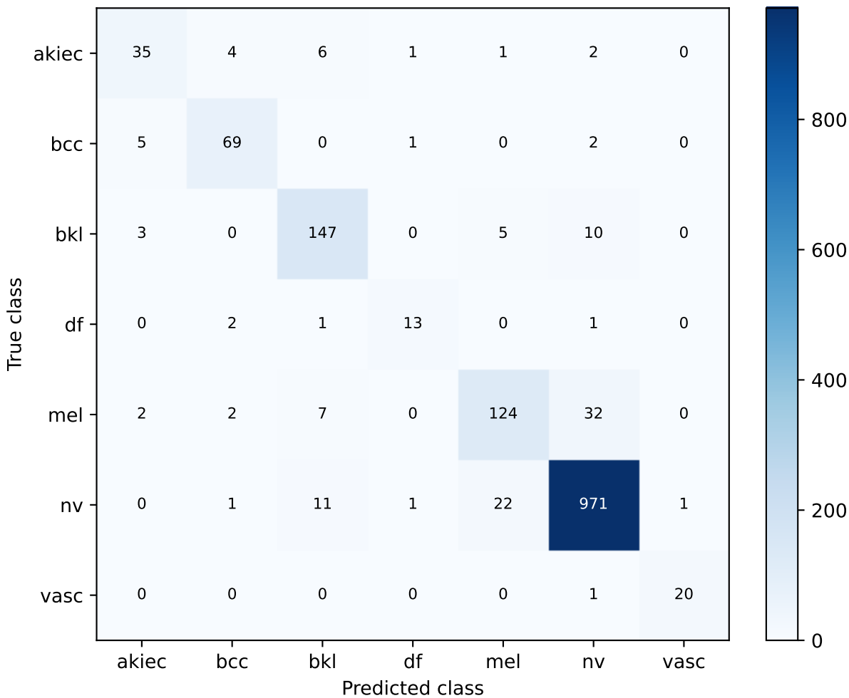
S42 crossfit_stacking | exploratory development Confusion matrix
