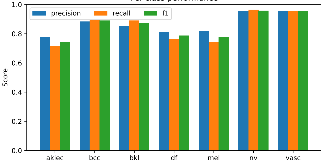
S42 crossfit_stacking | exploratory development Per-class performance
