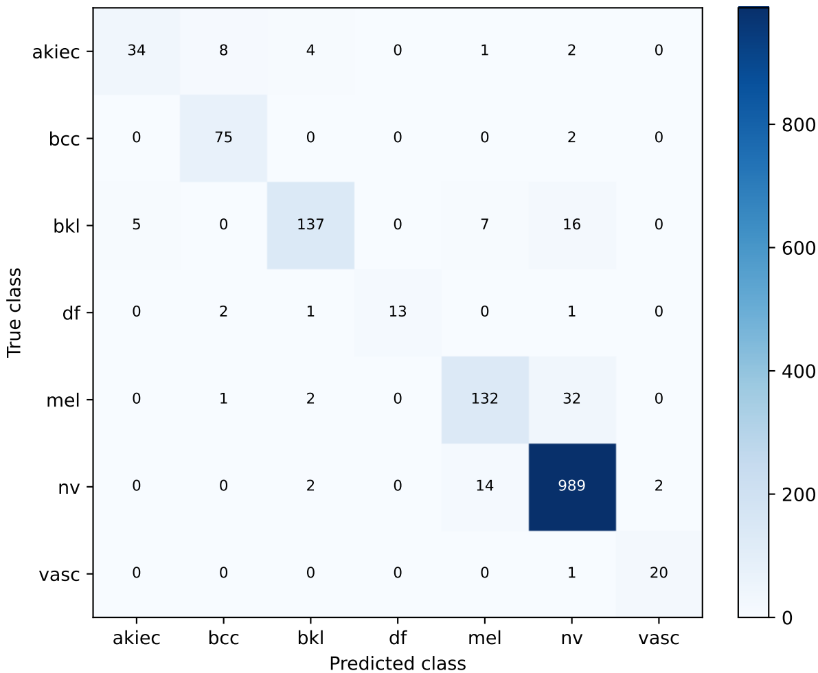
S42 equal_four_control | exploratory development Confusion matrix
