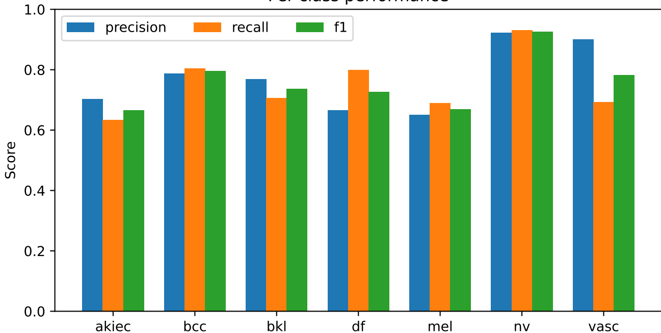
B3 fold-00 inner validation — epoch 21 Per-class performance
