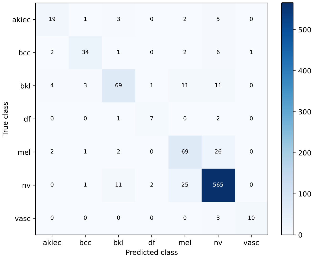
B3 fold-00 inner validation — epoch 26 Confusion matrix
