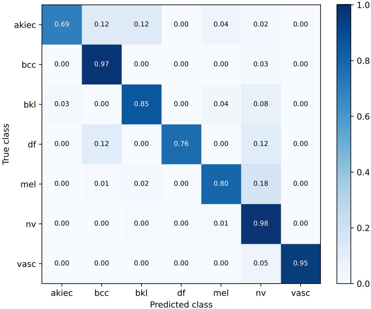
S47 hard_vote_probability_tiebreak | exploratory development Row-normalized confusion matrix
