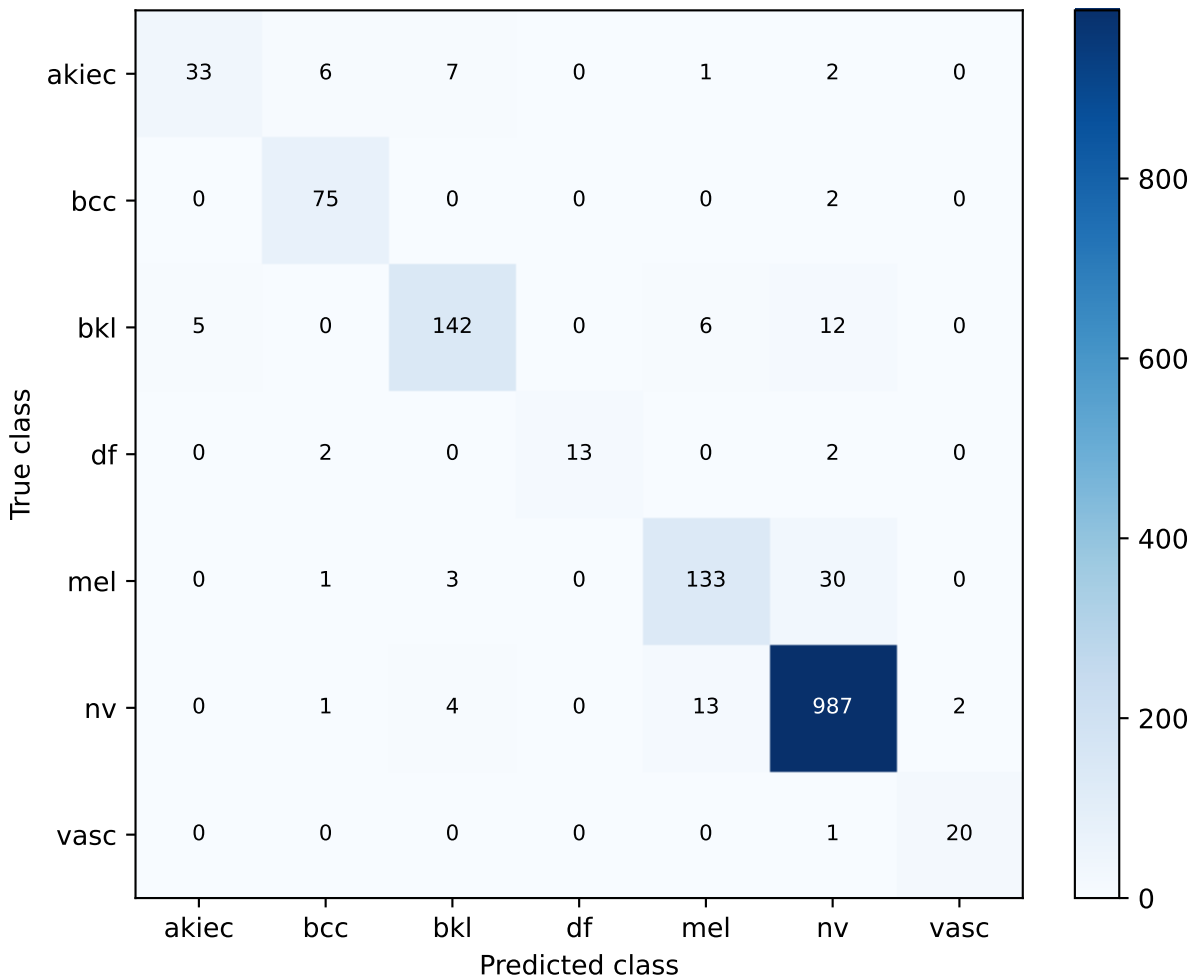
S48 trimmed_middle_two | exploratory development Confusion matrix
