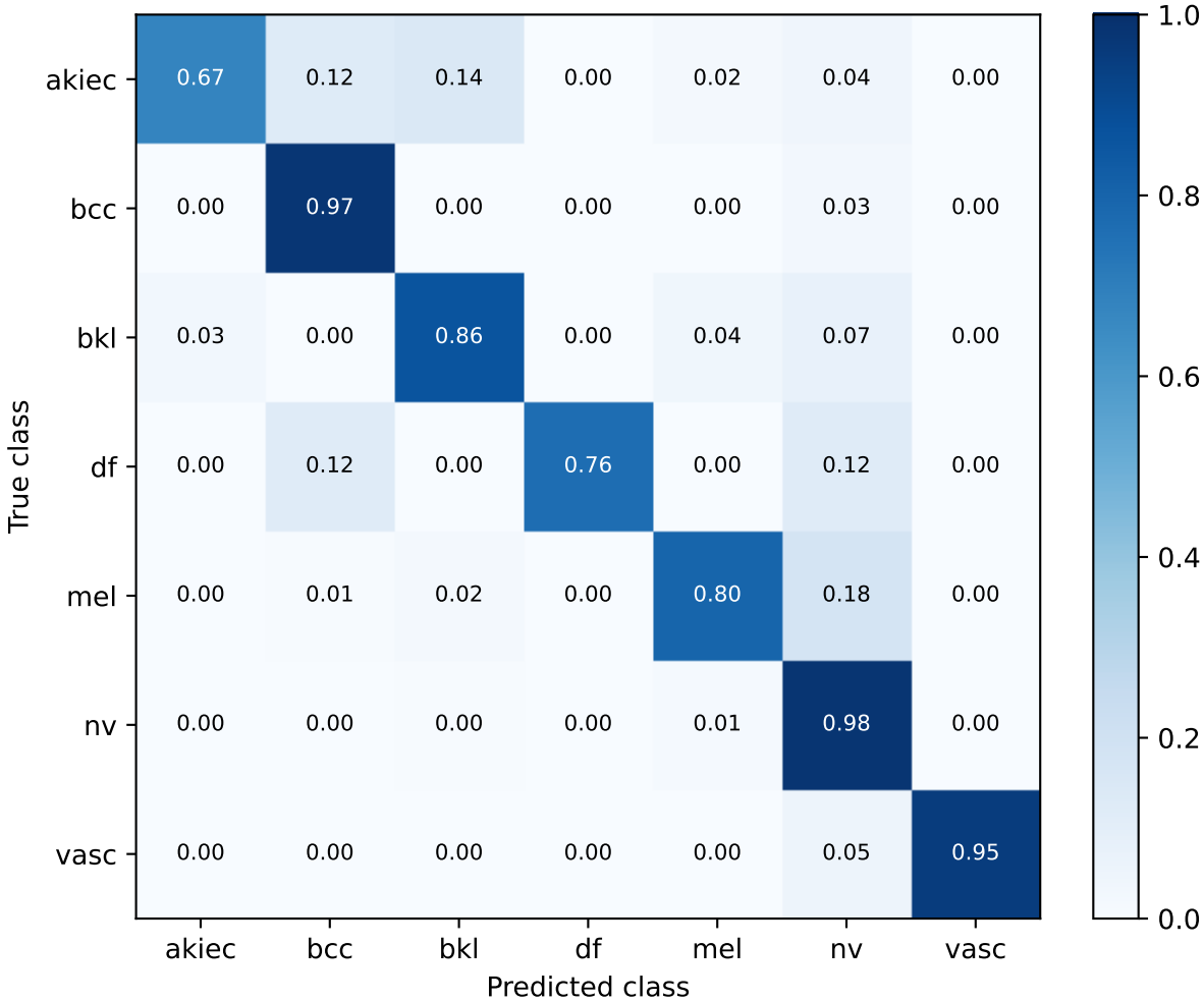
S48 trimmed_middle_two | exploratory development Row-normalized confusion matrix
