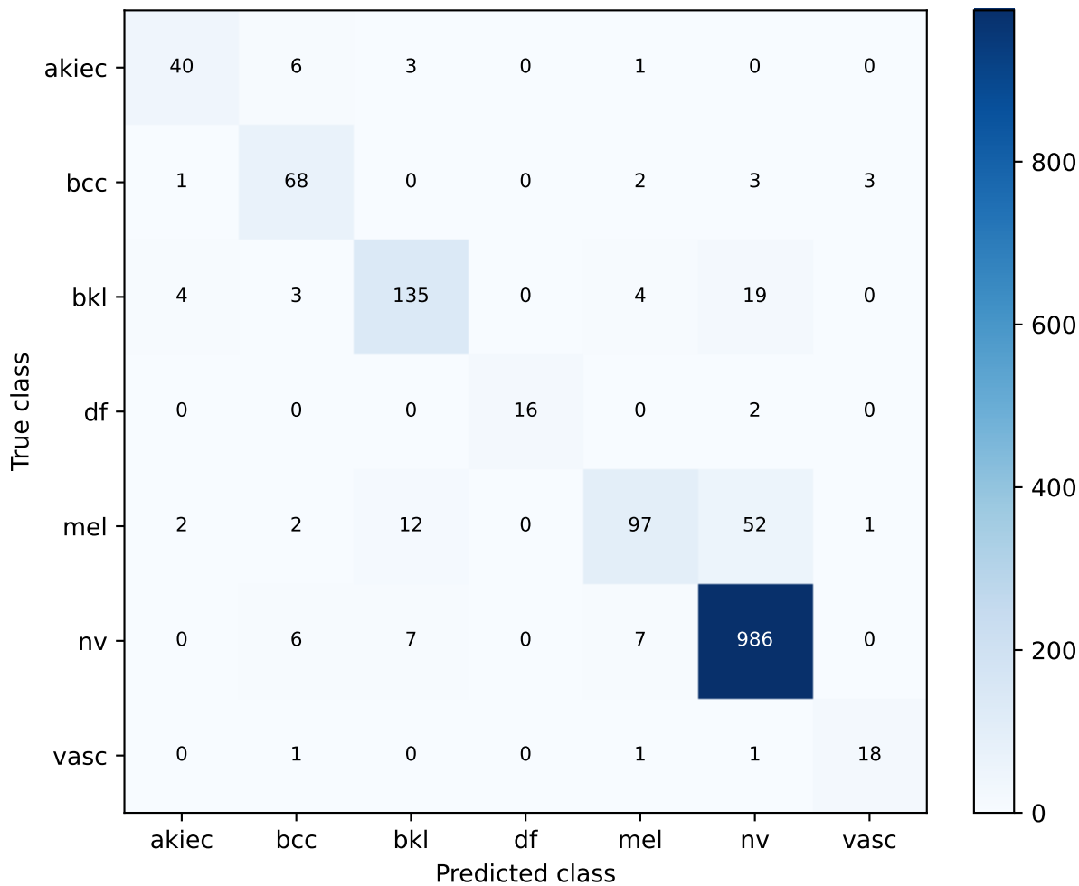
S41 fixed four-model equal fusion | strict development Confusion matrix
