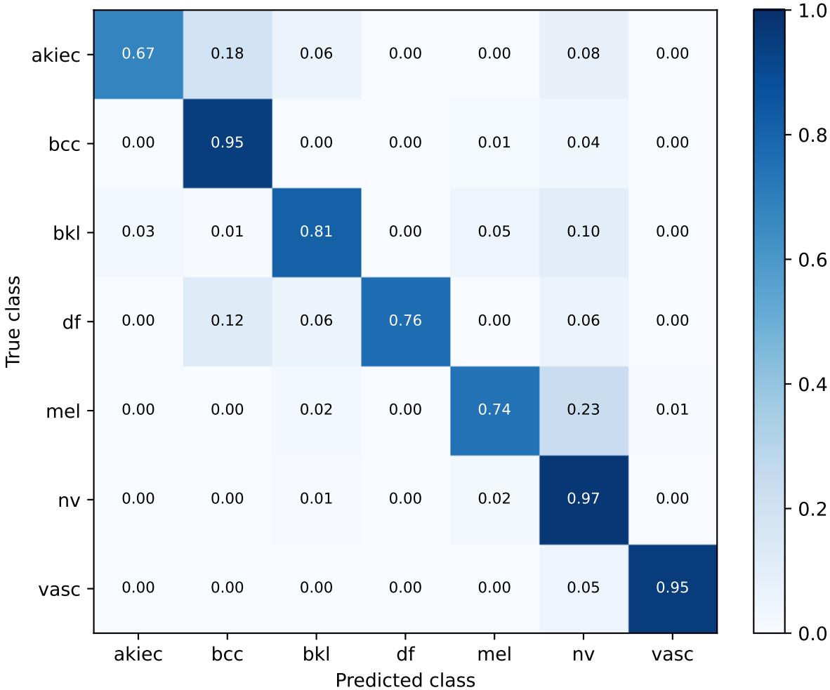
S13 tta | exploratory validation Row-normalized confusion matrix
