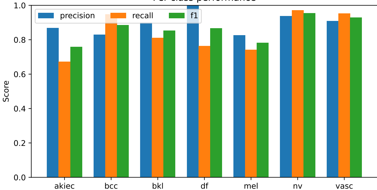
S13 tta | exploratory validation Per-class performance
