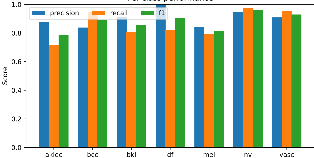
S13 identity_fp32 | exploratory validation Per-class performance
