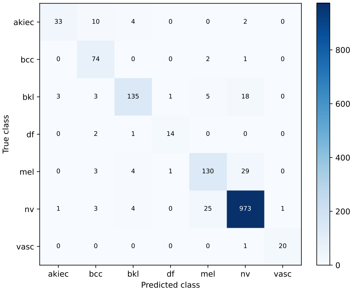
convnext_tiny | exploratory_image_level validation Confusion matrix
