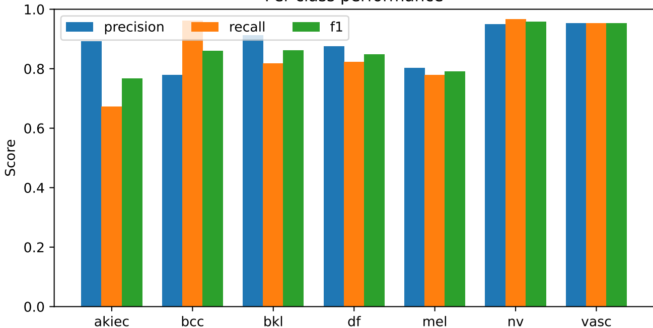
convnext_tiny | exploratory_image_level validation Per-class performance
