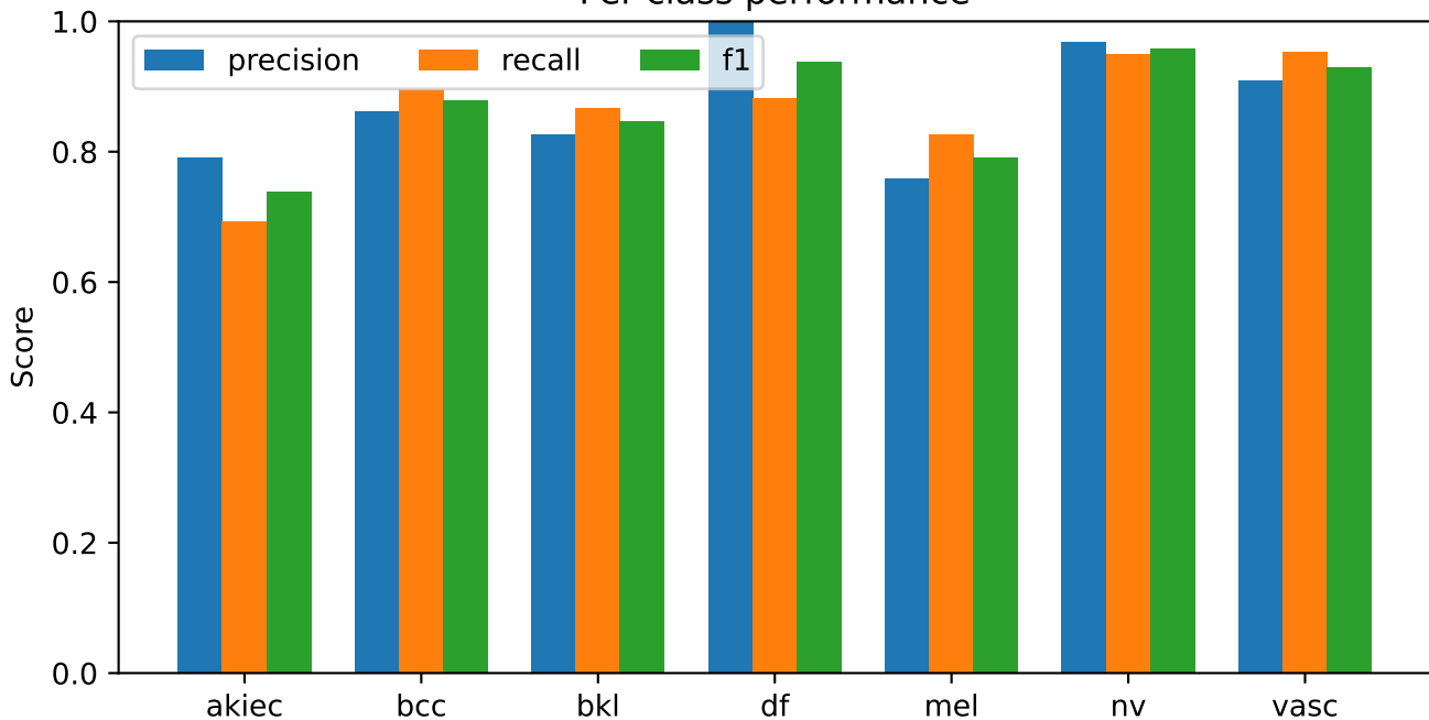
S06 ConvNeXt-Tiny | exploratory validation | macro-F1 winner Per-class performance
