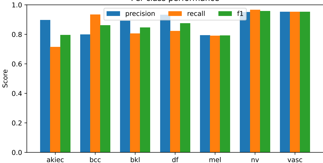
S09 fixed equal fusion | exploratory validation | no weight tuning Per-class performance
