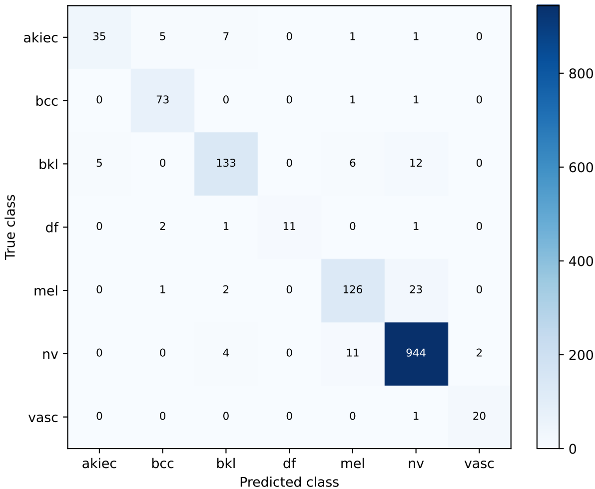
S70 S53 same-lesion multi-image | one fixed view per lesion Confusion matrix
