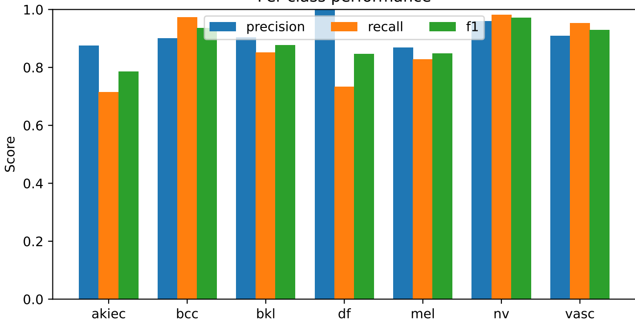
S70 S53 same-lesion multi-image | one fixed view per lesion Per-class performance
