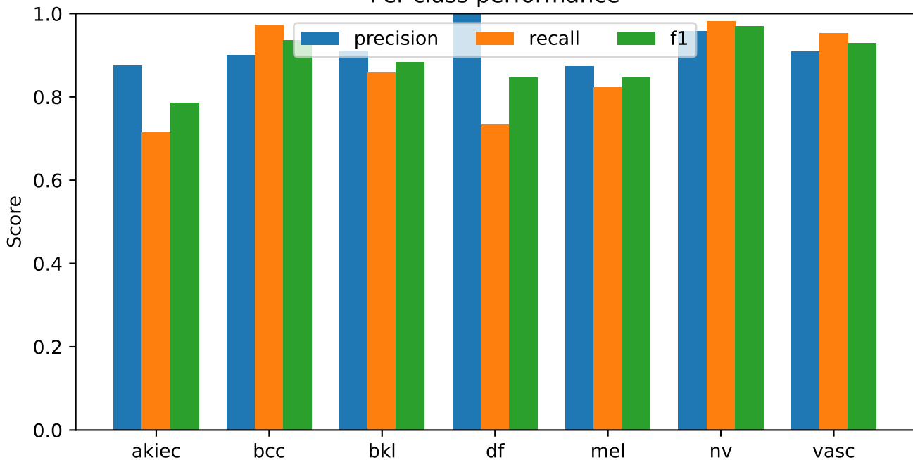
S70 S53 same-lesion multi-image | one score per lesion Per-class performance
