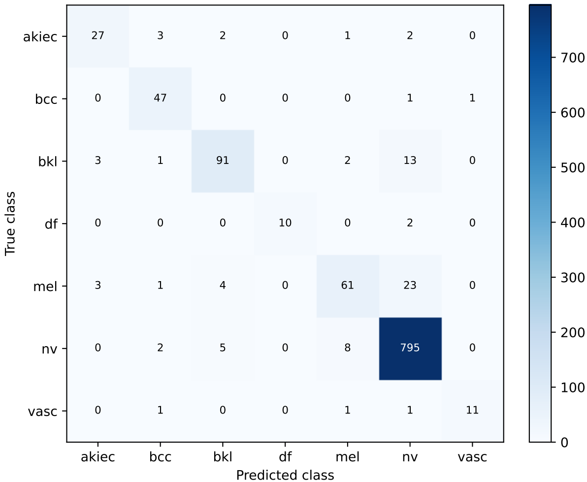
S71 S31 same-lesion multi-image | one score per lesion Confusion matrix
