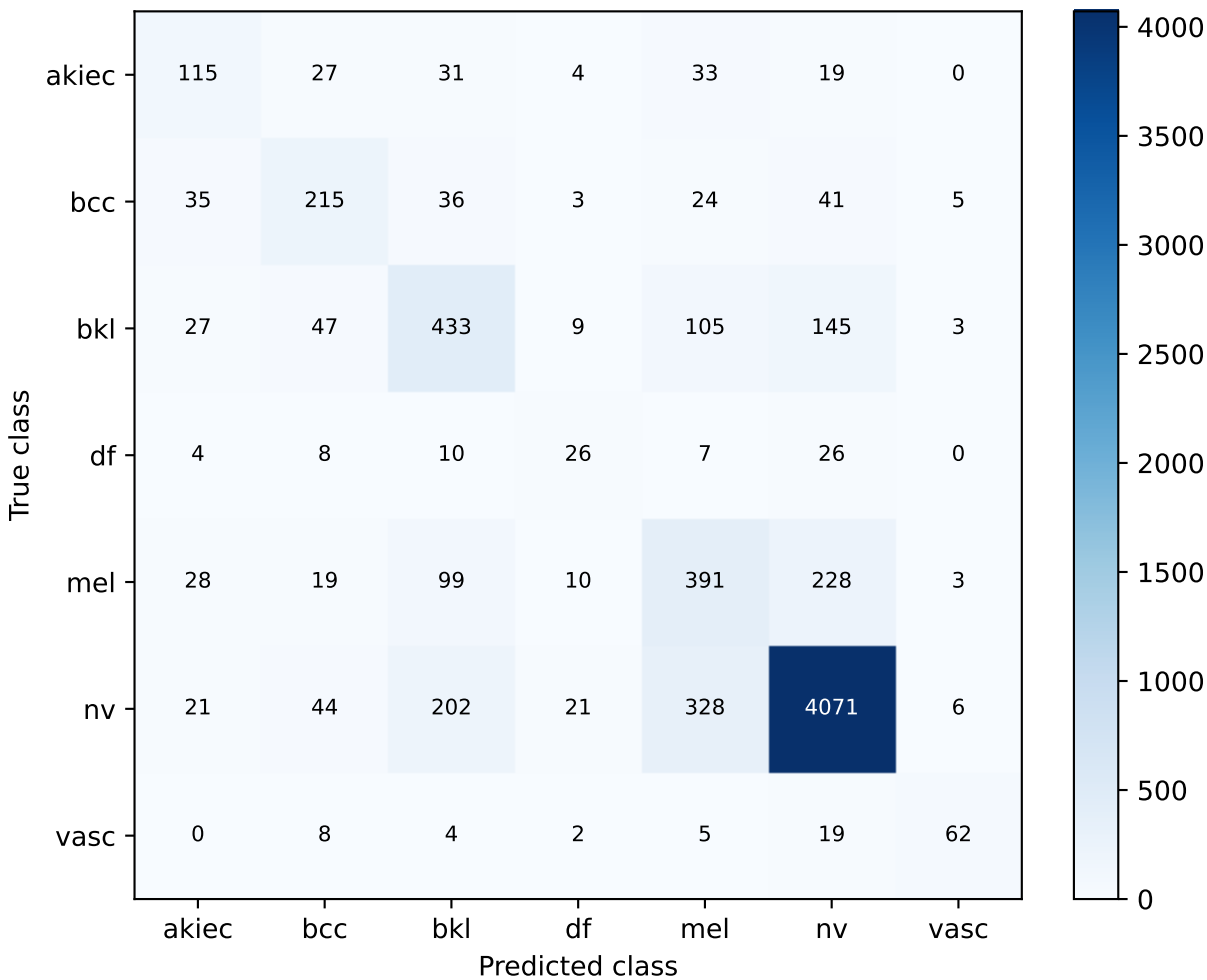
S72 linear | train-only lesion-group OOF Confusion matrix
