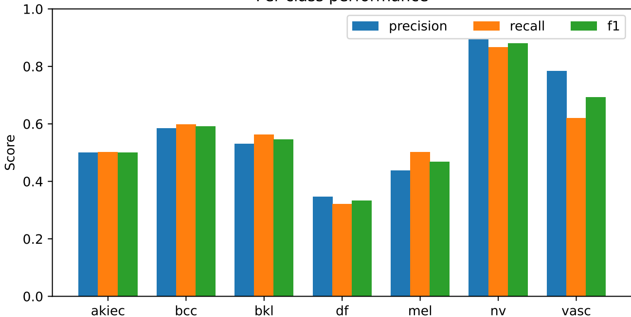
S72 linear | train-only lesion-group OOF Per-class performance
