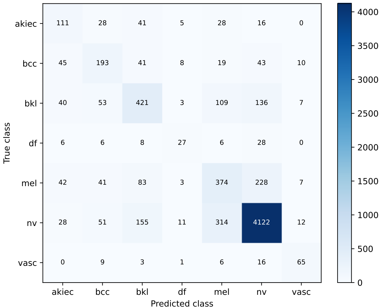
S72 rbf_nystroem | train-only lesion-group OOF Confusion matrix
